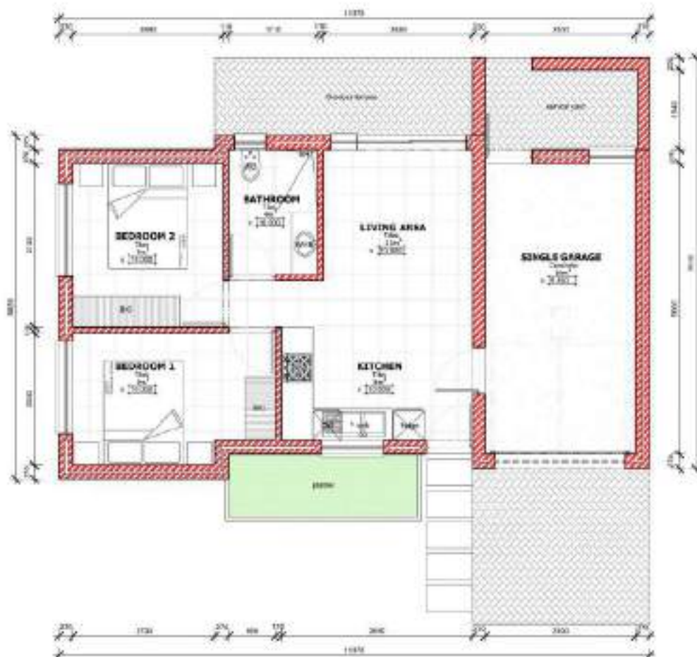
FLOOR PLAN_OPTION B_70 SQM SCALE 1:50
